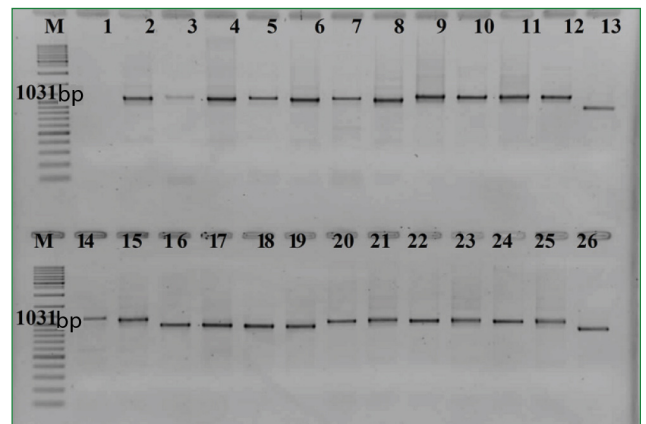
[Table/Fig-5]: Gel Image for PCR product shows :M: Marker (1Kb Gene Ruler™ DNA Ladder Mix, Fermentas®) 1: (-) control,2: (+) control, 3: T. rubrum 18, 4: T. rubrum 50, 5: T. rubrum 23, 6: T. rubrum 55, 7: T. rubrum 12, 8: T. Rubrum 4, 9: T.mentagrophytes 5, 10: T.mentagrophytes 7, 11: T.mentagrophytes 9,12: T.mentagrophytes 14, 13: A.niger 3, 14: T. mentagrophytes 13,15 : T.mentagrophytes 1, 16: T.rubrum 1,17: T.rubrum 5,18: T.rubrum 6, 19: T.rubrum 44, 20: E.floccosum 11, 21: E.floccosum 4, 22: E.floccosum 3, 23: E.floccosum 2, 24: E.floccosum 13, 25: E.floccosum 5, 26: A.niger 11
